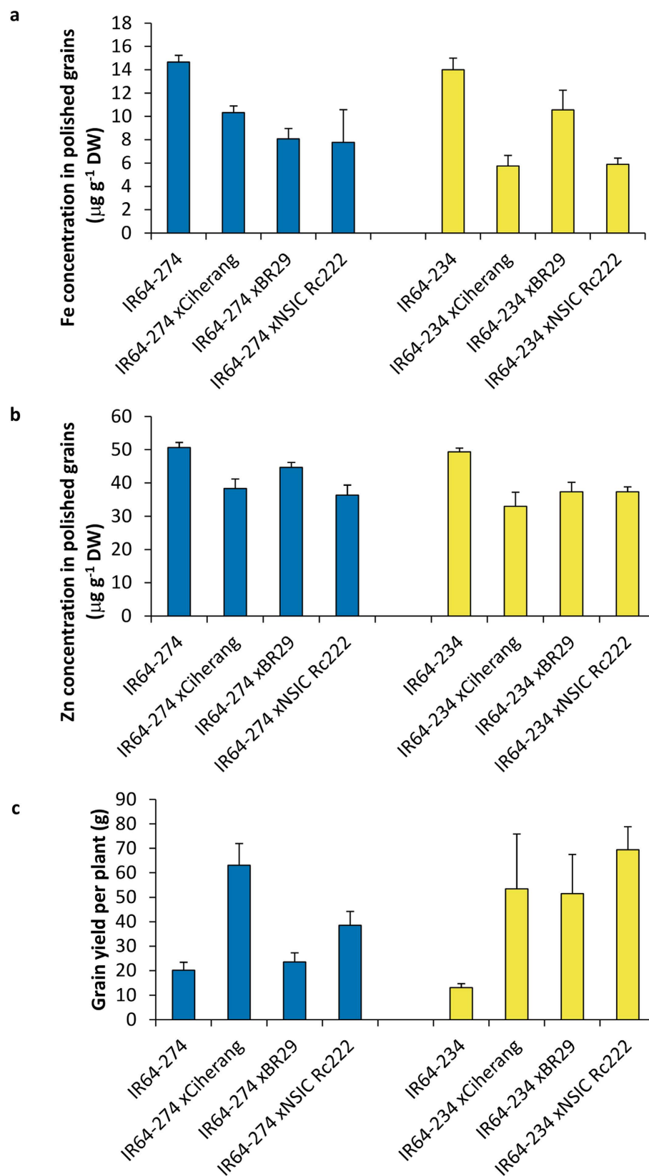
Figure 6. Stability of Fe and Zn concentrations in different genetic backgrounds. (a) Fe concentration ( \mu\text{g g}^{-1} DW) of polished seeds harvested from F_1 plants derived from crossing between lead events and popular varieties. (b) Zn concentration ( \mu\text{g g}^{-1} DW) of polished seeds harvested from F_1 plants derived from crossing between lead events and popular varieties. (c) Grain yield of F_1 plants derived from crossing between lead event and popular varieties. Bars represent the means \pm s.d. of three replicates.
