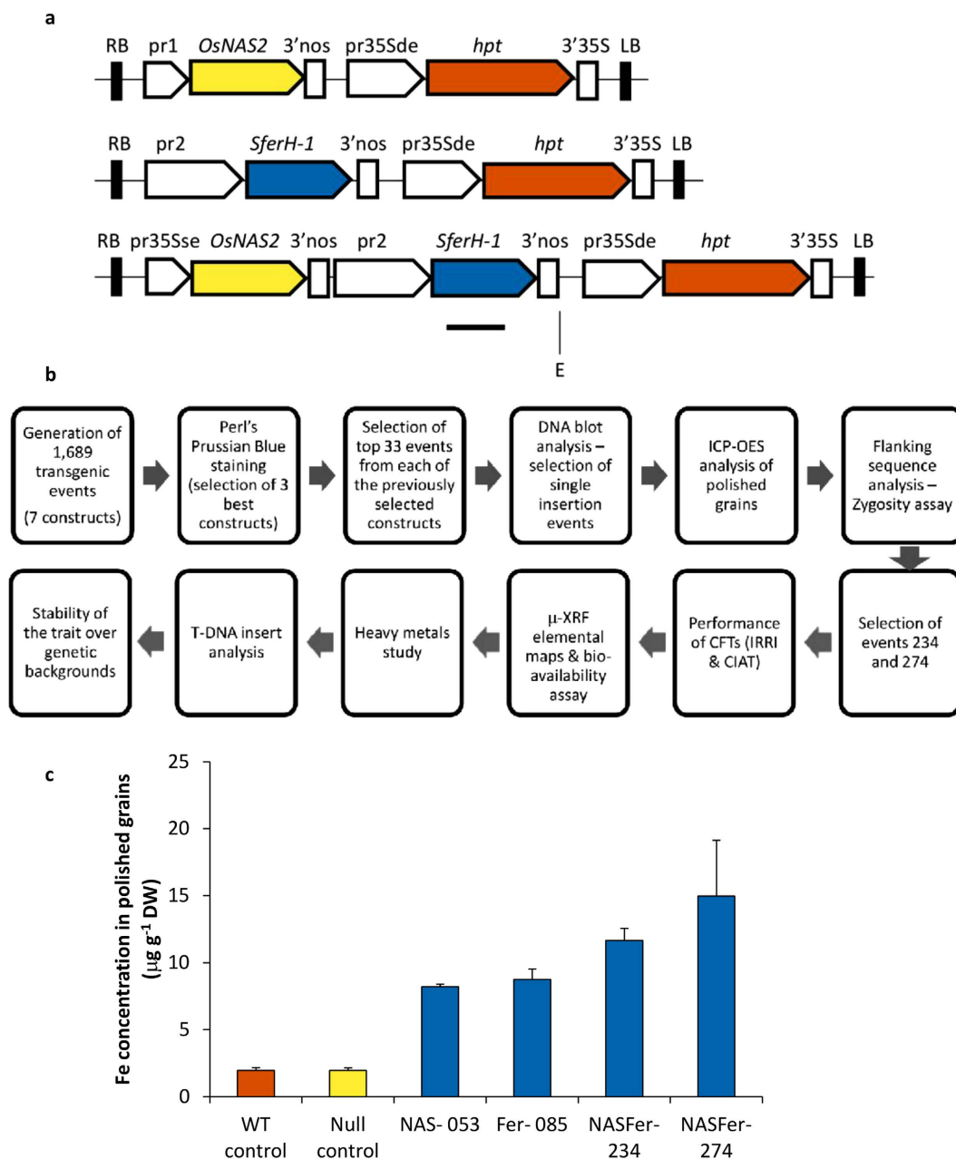
Figure 1. Strategy for the development of biofortified high-iron rice and the Fe concentration achieved in T 2 polished seeds. (a) Schematic diagram of the T-DNA constructs prepared for rice transformation for the purposes of our study. RB and LB represent the right and left borders of the T-DNA, respectively; pr1: represents the constitutive promoters pr35S with single enhancer (pr35Sse), maize ubiquitin promoter, or rice endosperm-specific promoter glutelinB1; pr2: represents the rice endosperm-specific promoters glutelinB1 or glutelinA2; pr35Sde represents the constitutive promoter pr35S with double enhancer; OsNAS2 : Oryza sativa nicotianamine synthase 2; SferH-1 : Glycine max ferritin subunit H-1; hpt : hygromycin phosphotransferase; 3'nos: 3'UTR of nopaline synthase; 3'35S: 3'UTR of 35S cauliflower mosaic virus gene. The horizontal line below SferH-1 represents the deduced hybridization position of the digoxigenin-labeled cDNA probe; E: EcoRI . (b) Flow-chart displaying the steps that have been followed for the development of biofortified high-Fe/-Zn rice. (c) Fe concentration (μg g -1 DW) of polished seeds harvested from T 1 homozygous plants of representative NAS, Fer, and NASFer events, null segregant, and non-transformed rice under greenhouse conditions. Bars represent the means ± s.d. of three replicates.
